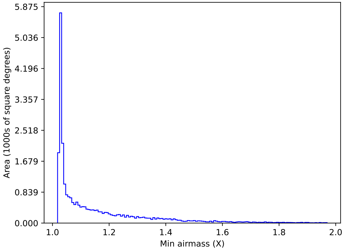
no_magell_roll_v3.4_10yrs All sky z band: Min airmass
