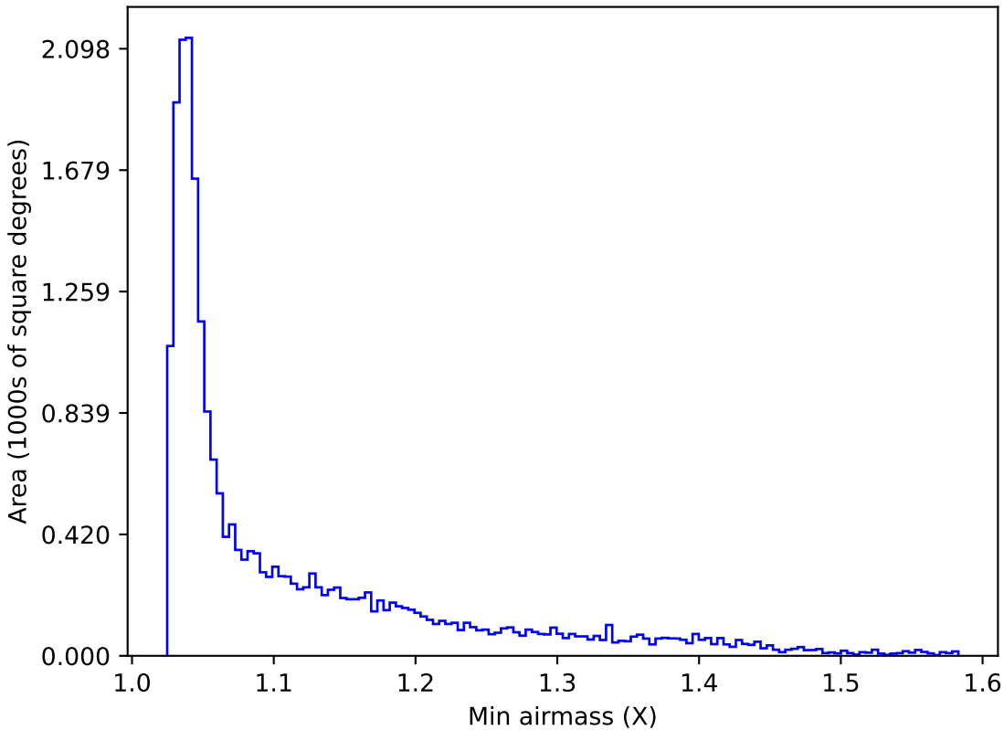
no_magell_roll_v3.4_10yrs All sky u band: Min airmass
