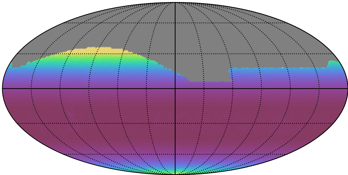
no_magell_roll_v3.4_10yrs All sky r band: Min airmass
