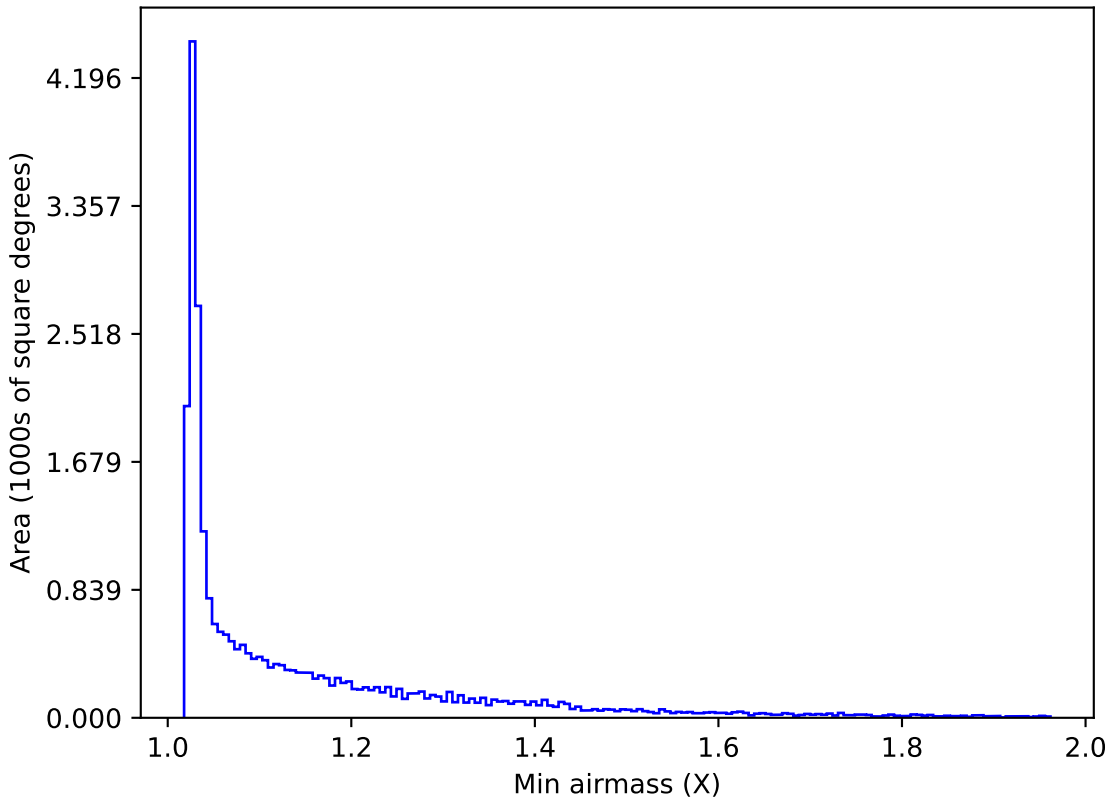
no_magell_roll_v3.4_10yrs All sky r band: Min airmass
