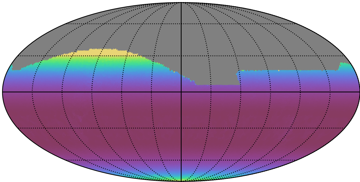
no_magell_roll_v3.4_10yrs All sky i band: Min airmass
