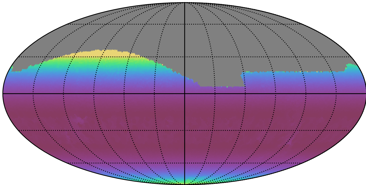
no_magell_roll_v3.4_10yrs All sky g band: Min airmass
