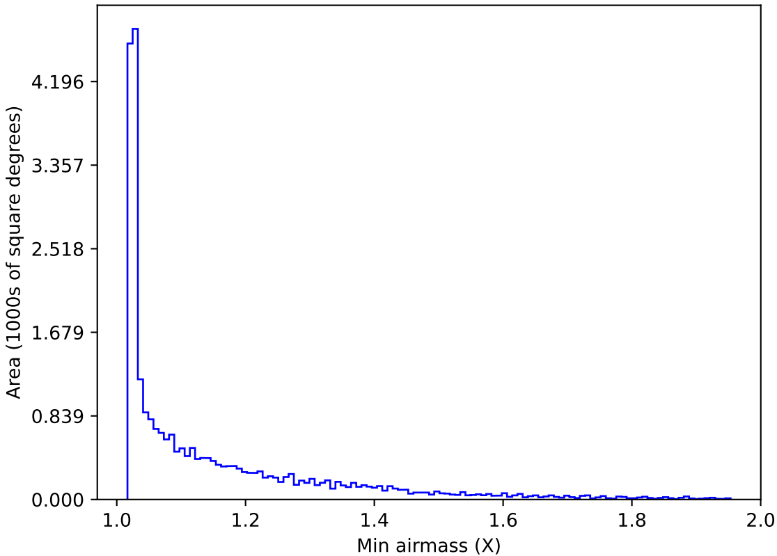
no_magell_roll_v3.4_10yrs All sky all bands: Min airmass
