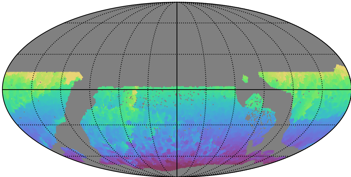
no_magell_roll_v3.4_10yrs WFD all bands: Min HA
