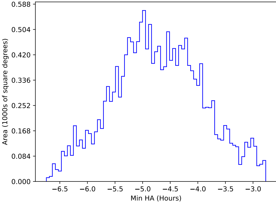
no_magell_roll_v3.4_10yrs WFD all bands: Min HA
