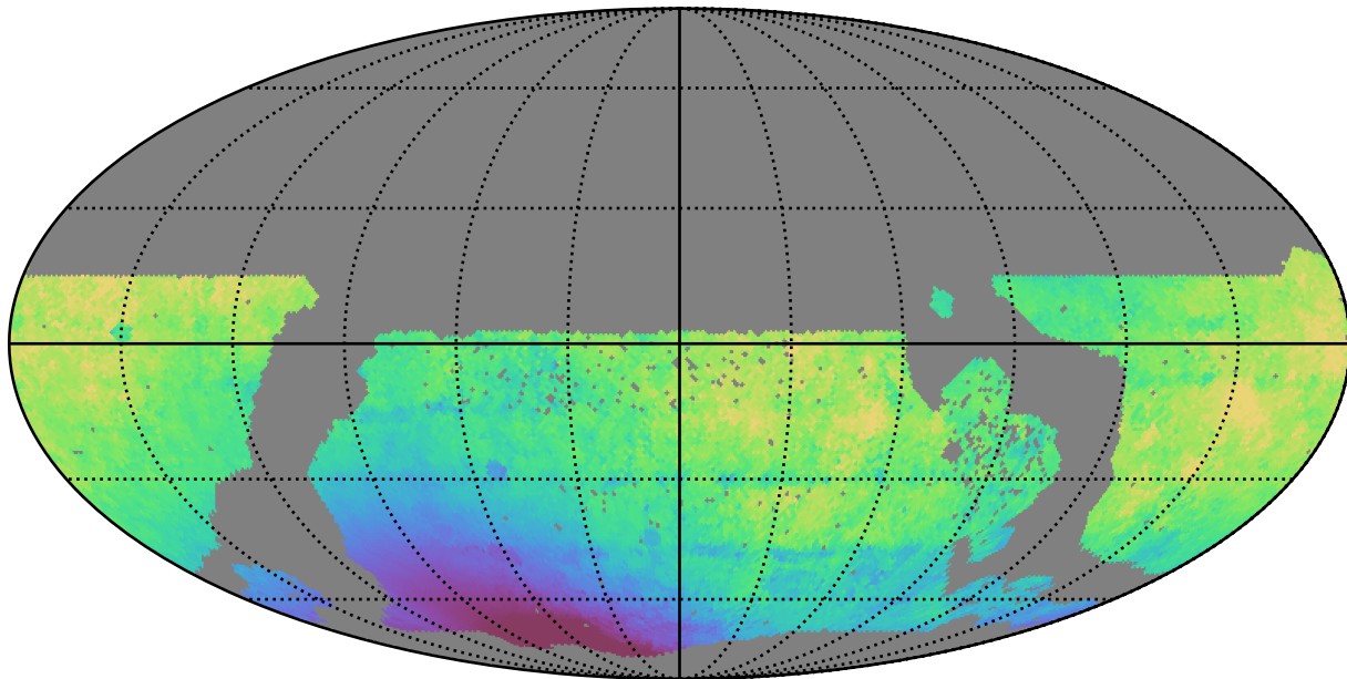
no_magell_roll_v3.4_10yrs WFD z band: Median solarElong
