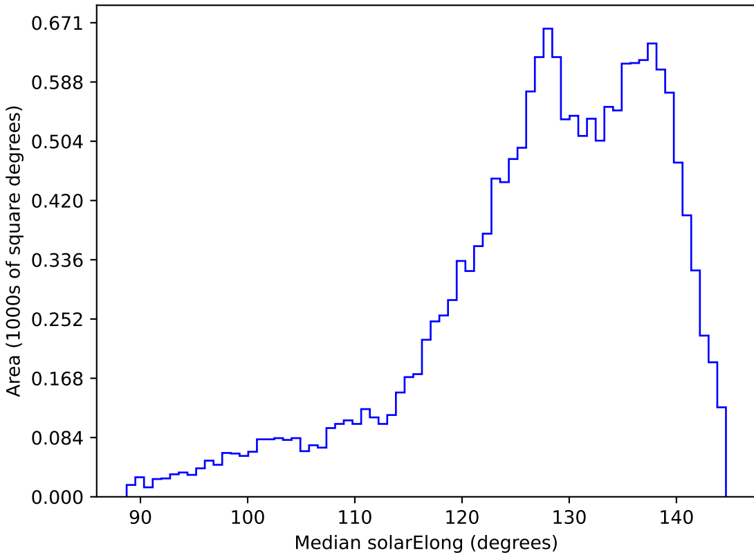
no_magell_roll_v3.4_10yrs WFD z band: Median solarElong
