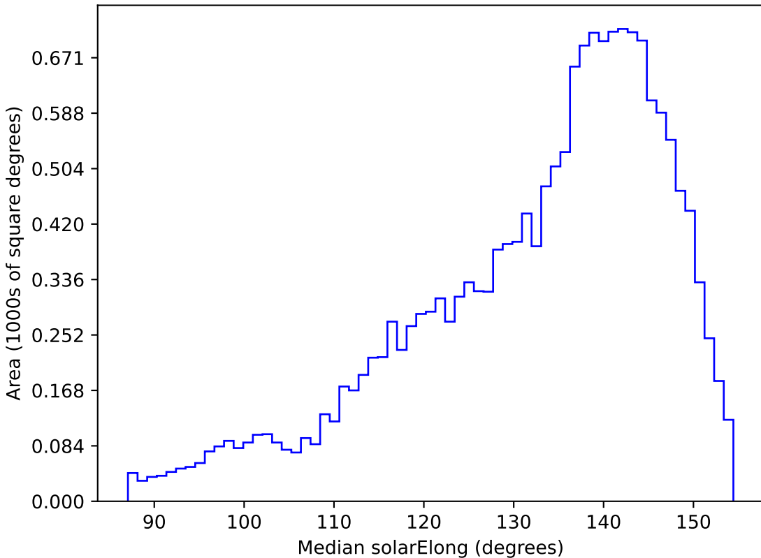
no_magell_roll_v3.4_10yrs WFD u band: Median solarElong
