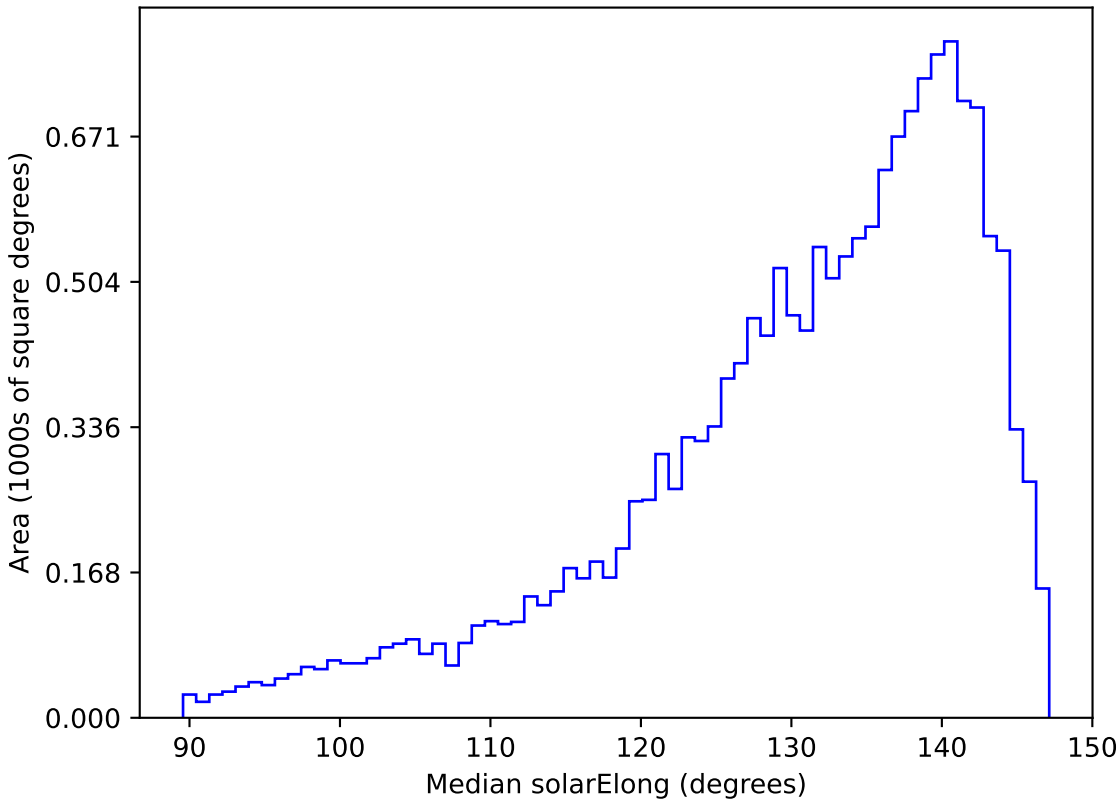
no_magell_roll_v3.4_10yrs WFD r band: Median solarElong
