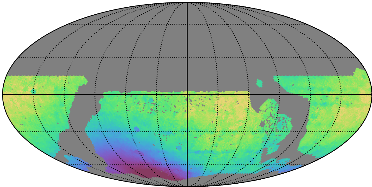
no_magell_roll_v3.4_10yrs WFD i band: Median solarElong
