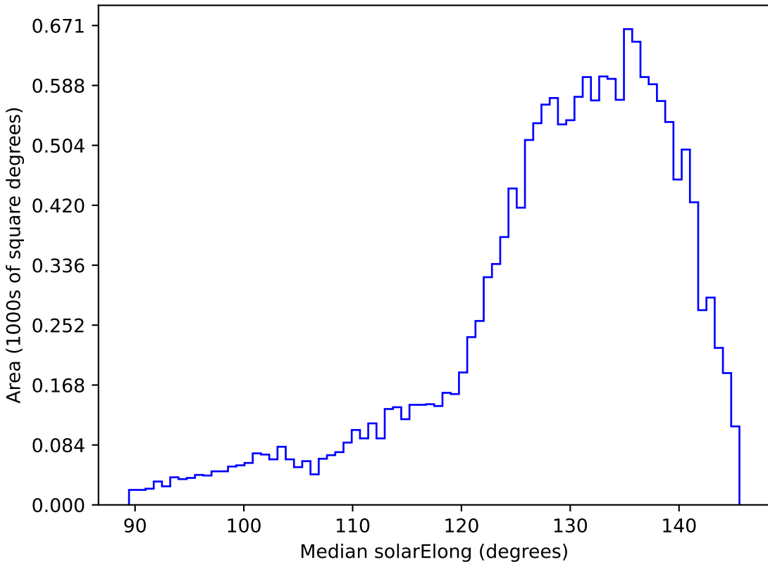
no_magell_roll_v3.4_10yrs WFD i band: Median solarElong
