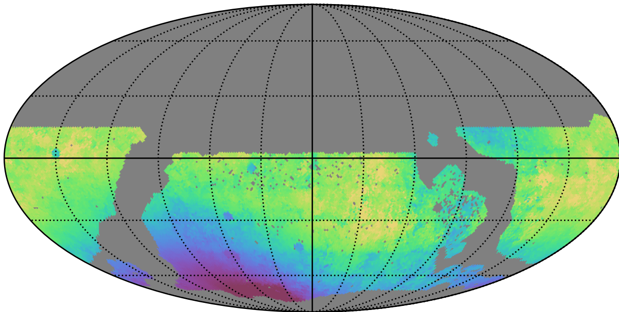
no_magell_roll_v3.4_10yrs WFD g band: Median solarElong
