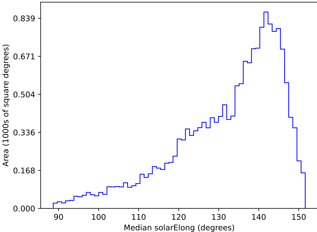
no_magell_roll_v3.4_10yrs WFD g band: Median solarElong
