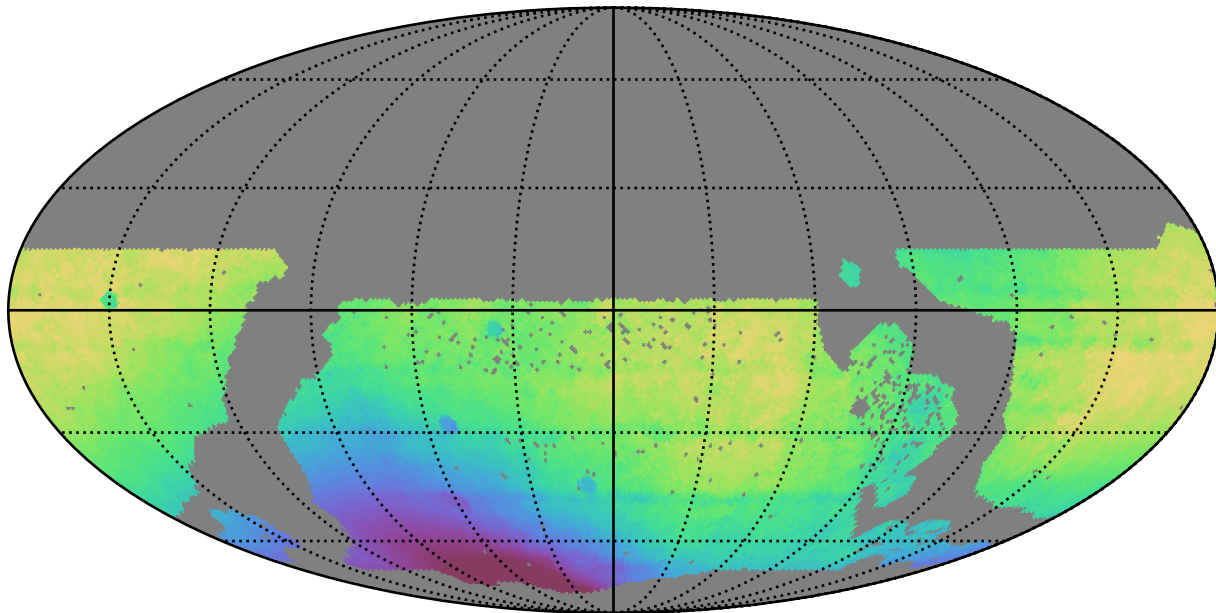
no_magell_roll_v3.4_10yrs WFD all bands: Median solarElong
