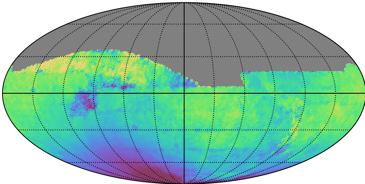
no_magell_roll_v3.4_10yrs All sky z band: Median solarElong
