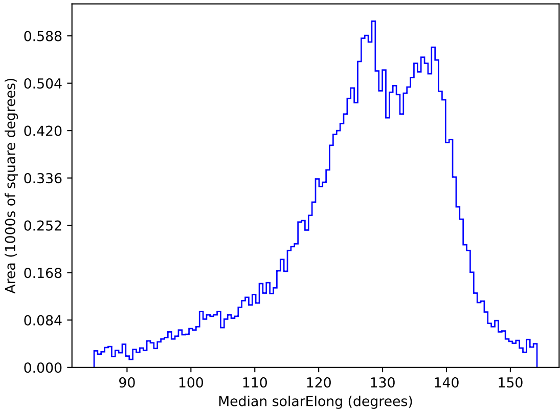
no_magell_roll_v3.4_10yrs All sky z band: Median solarElong
