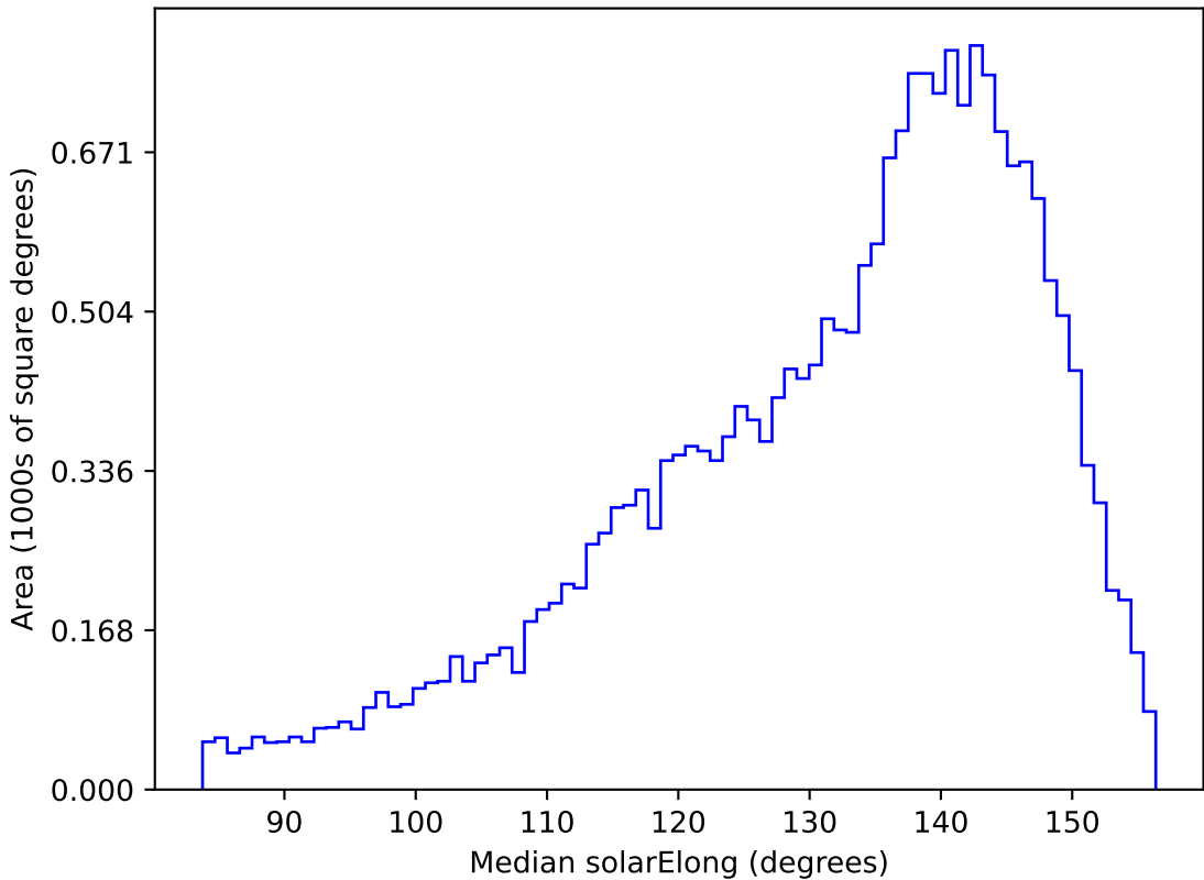
no_magell_roll_v3.4_10yrs All sky u band: Median solarElong
