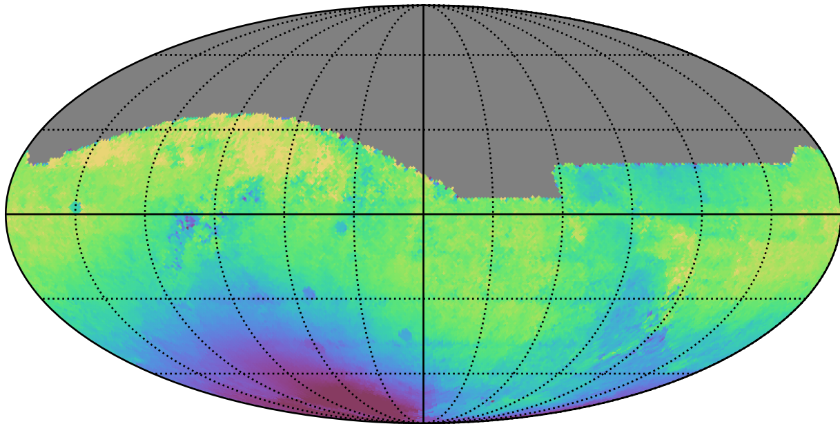
no_magell_roll_v3.4_10yrs All sky r band: Median solarElong
