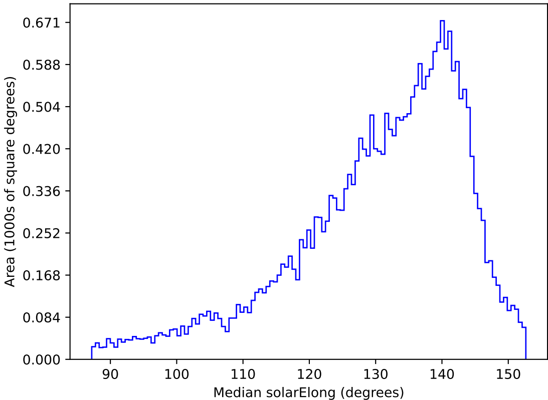
no_magell_roll_v3.4_10yrs All sky r band: Median solarElong
