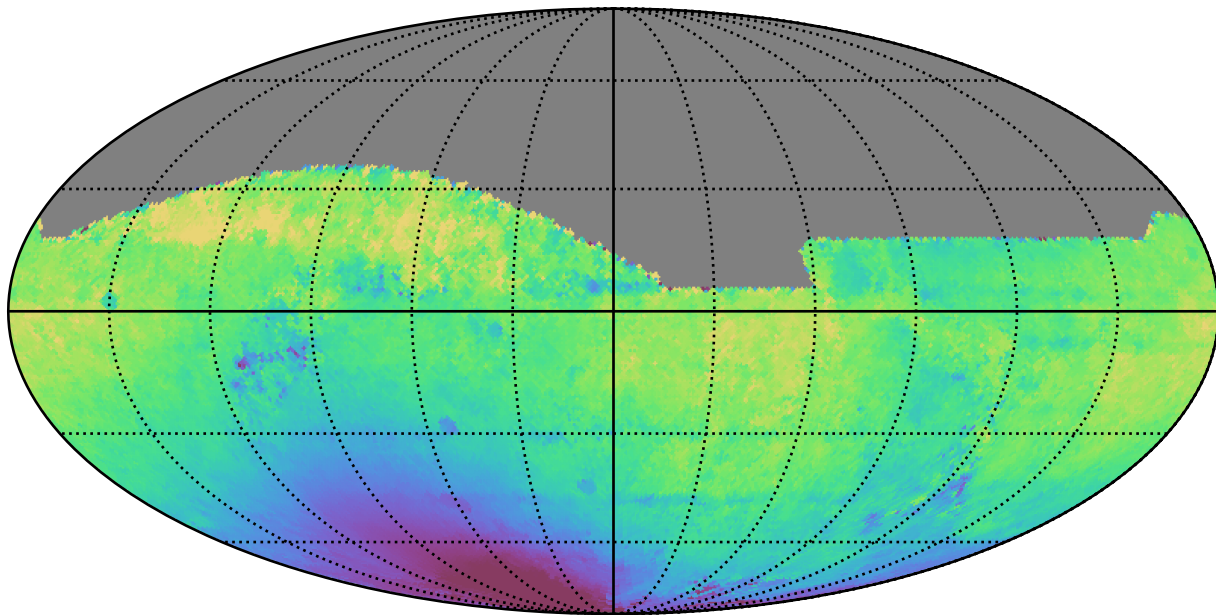
no_magell_roll_v3.4_10yrs All sky i band: Median solarElong
