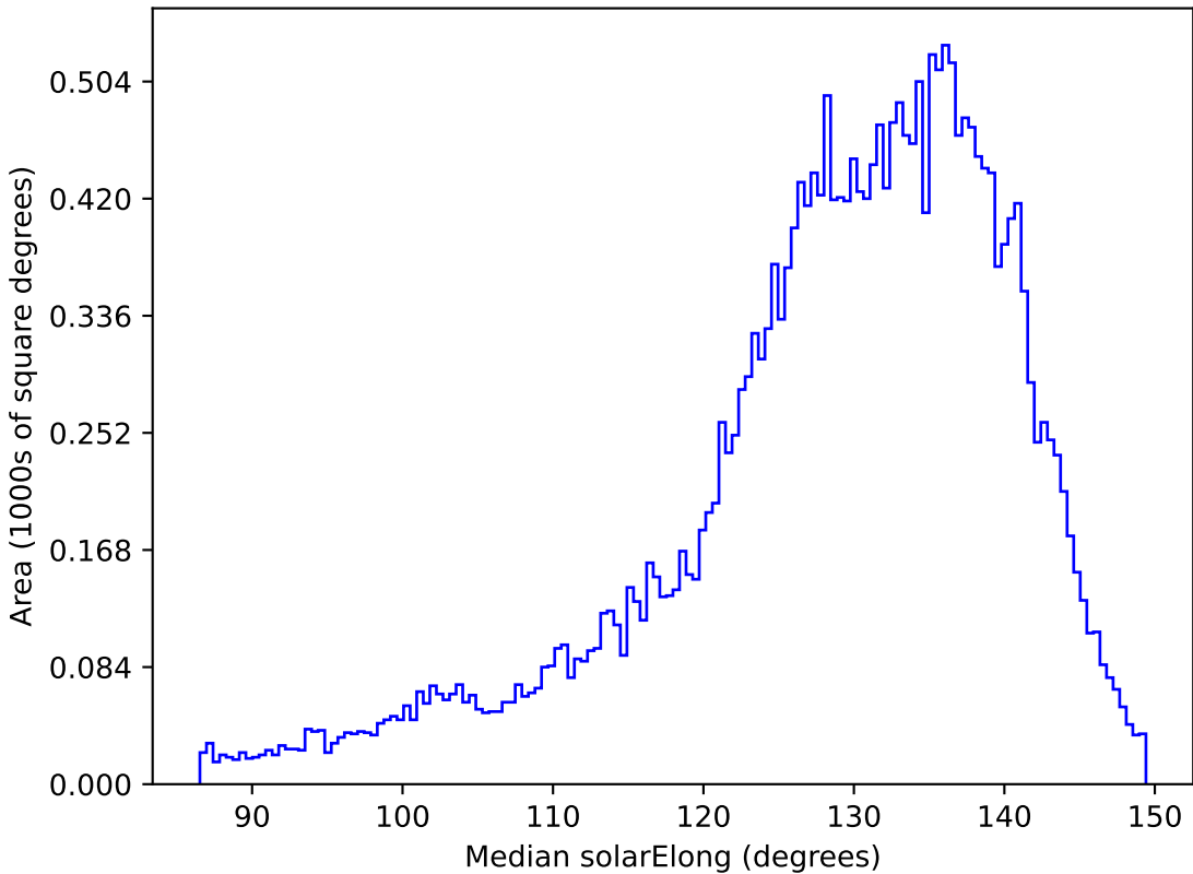
no_magell_roll_v3.4_10yrs All sky i band: Median solarElong
