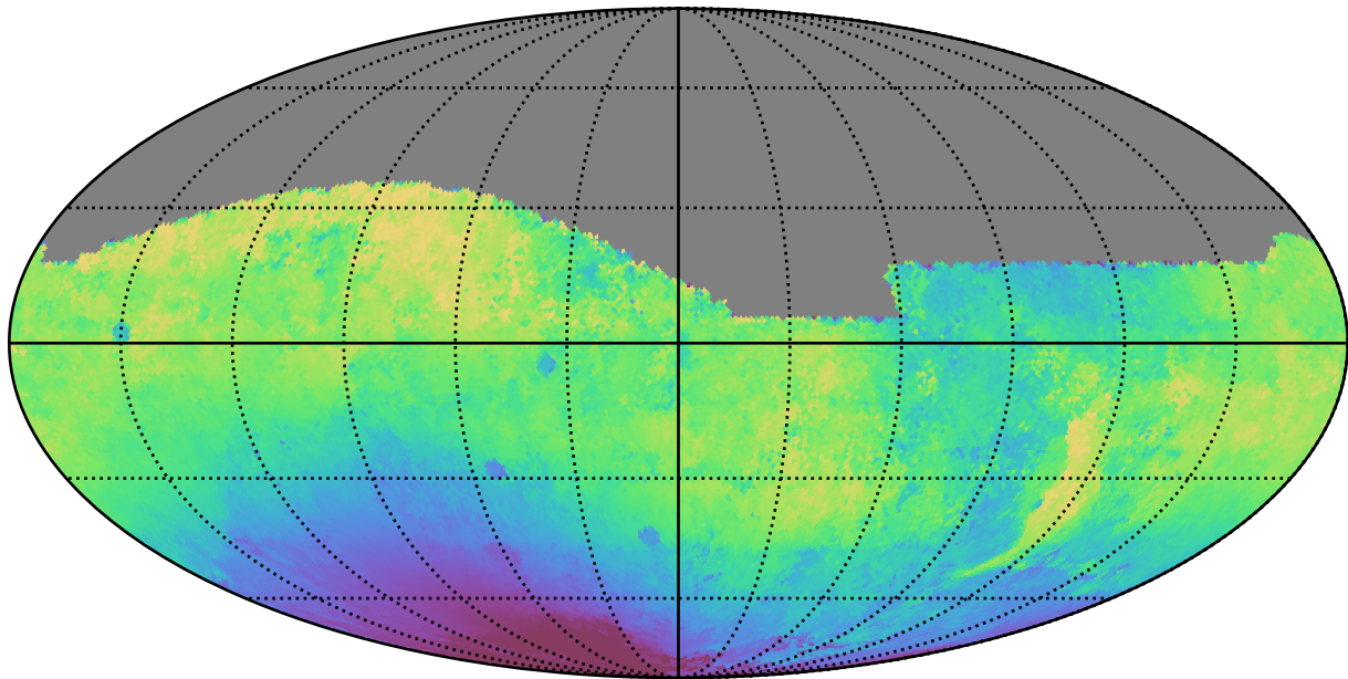
no_magell_roll_v3.4_10yrs All sky g band: Median solarElong
