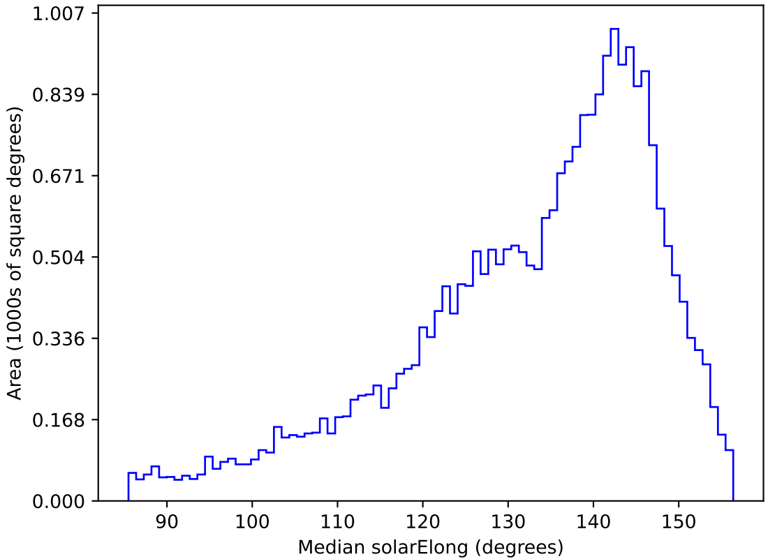
no_magell_roll_v3.4_10yrs All sky g band: Median solarElong
