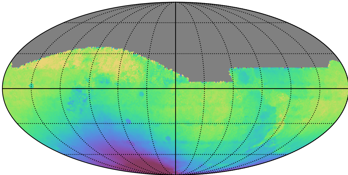
no_magell_roll_v3.4_10yrs All sky all bands: Median solarElong
