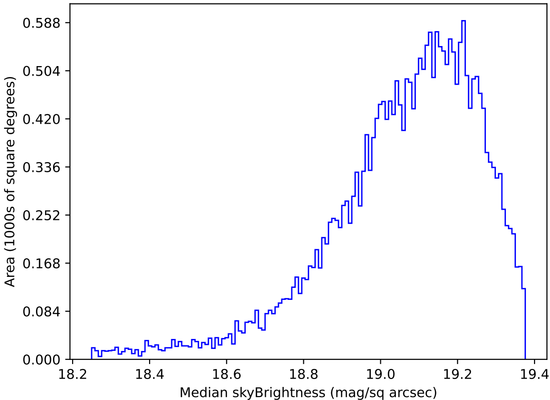
no_magell_roll_v3.4_10yrs Yr 1 z band: Median skyBrightness
