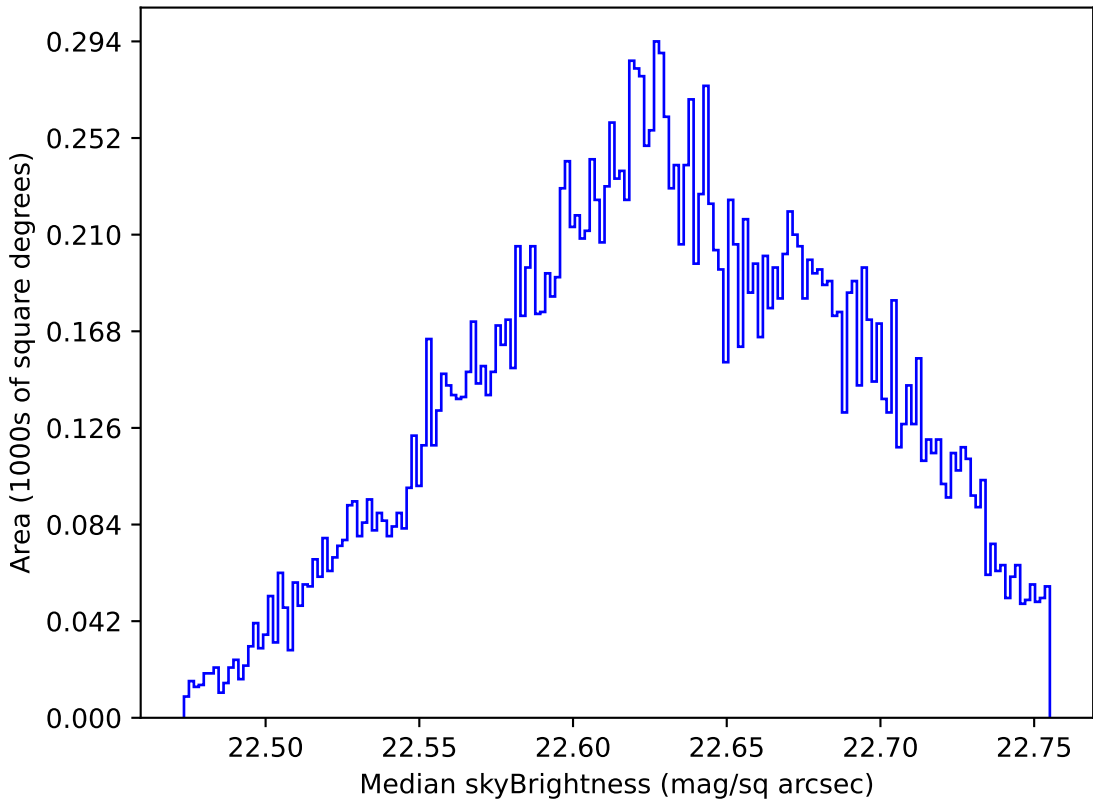
no_magell_roll_v3.4_10yrs Yr 1 u band: Median skyBrightness
