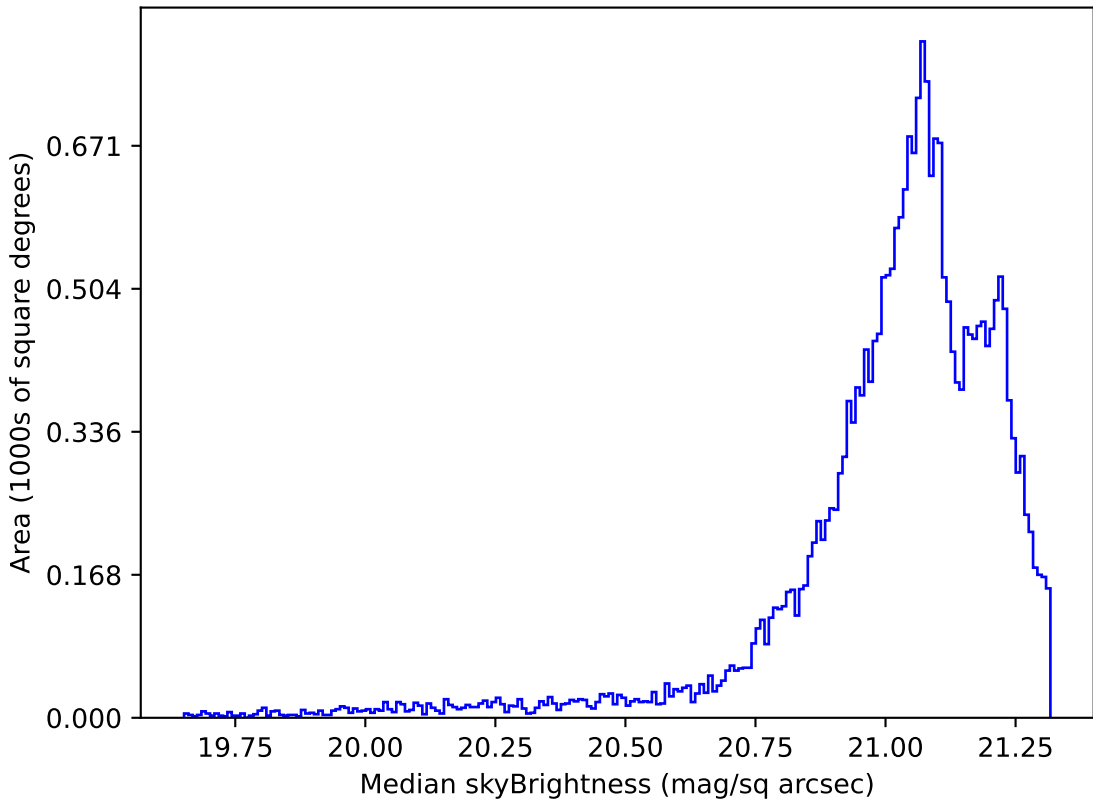
no_magell_roll_v3.4_10yrs Yr 1 r band: Median skyBrightness
