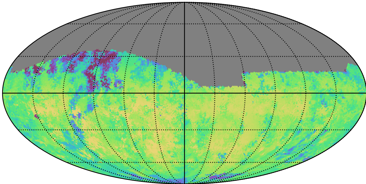
no_magell_roll_v3.4_10yrs Yr 1 i band: Median skyBrightness
