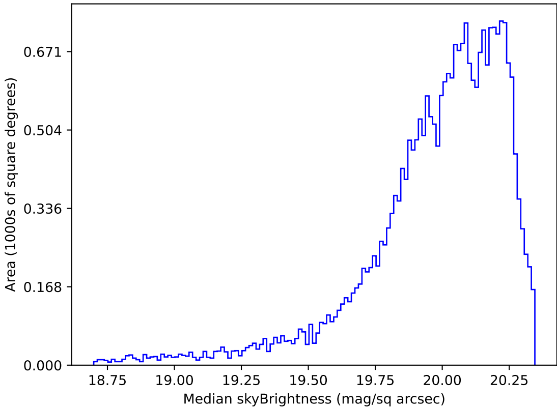
no_magell_roll_v3.4_10yrs Yr 1 i band: Median skyBrightness
