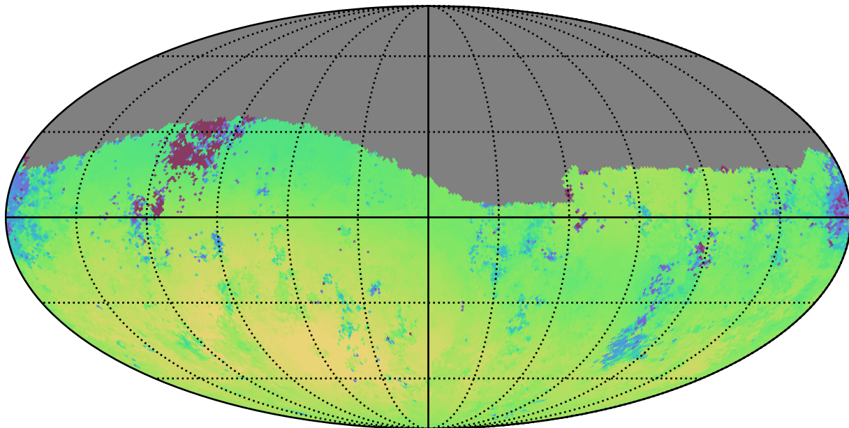
no_magell_roll_v3.4_10yrs Yr 1 g band: Median skyBrightness
