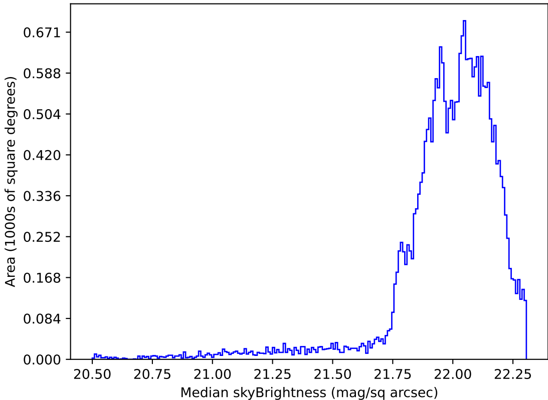
no_magell_roll_v3.4_10yrs Yr 1 g band: Median skyBrightness
