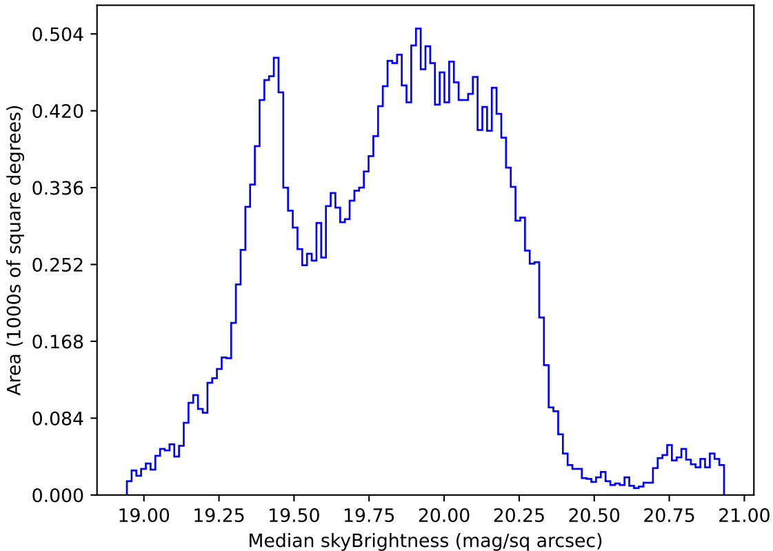
no_magell_roll_v3.4_10yrs Yr 1 all bands: Median skyBrightness
