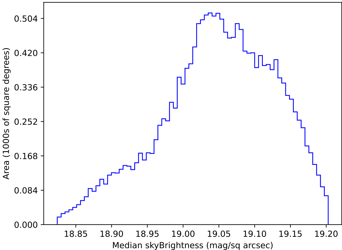
no_magell_roll_v3.4_10yrs WFD z band: Median skyBrightness
