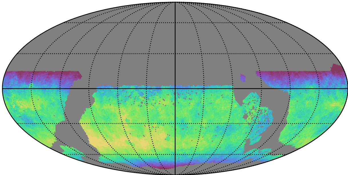
no_magell_roll_v3.4_10yrs WFD y band: Median skyBrightness
