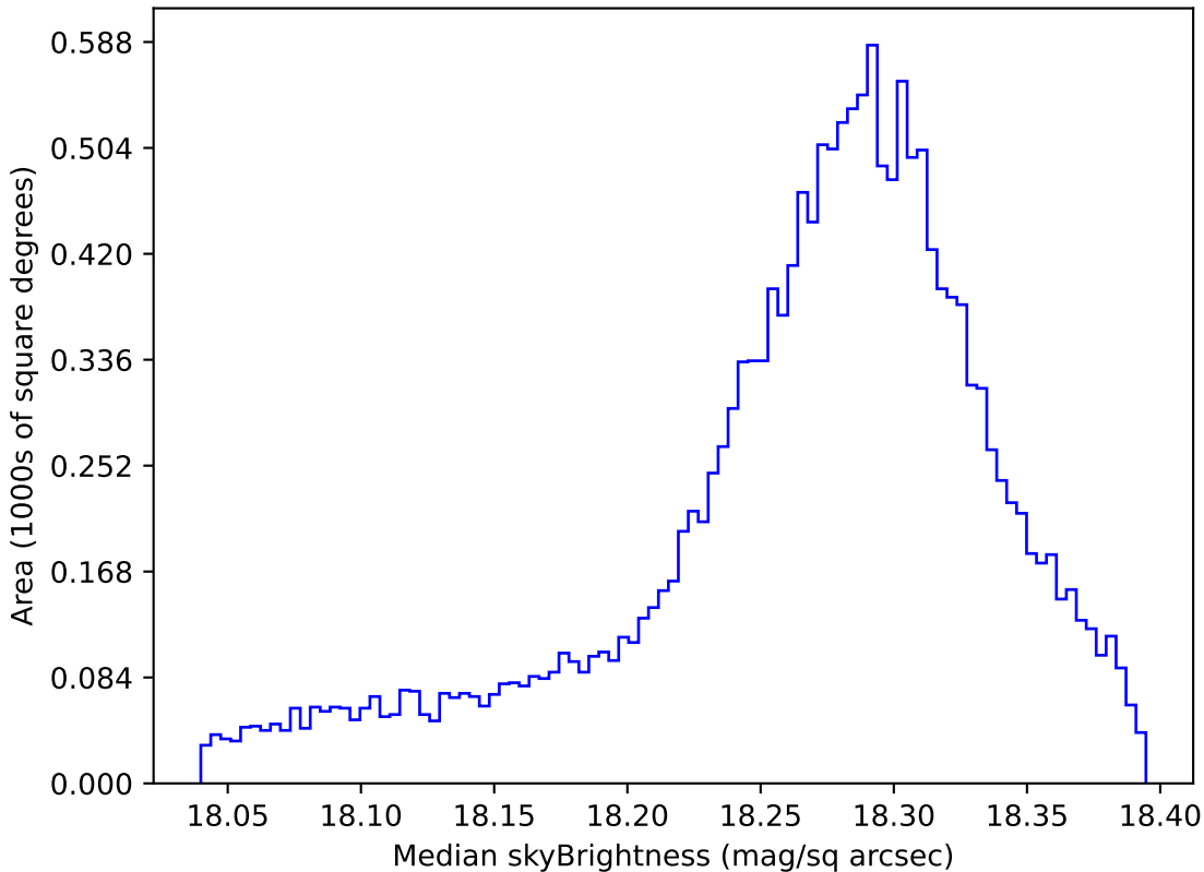
no_magell_roll_v3.4_10yrs WFD y band: Median skyBrightness
