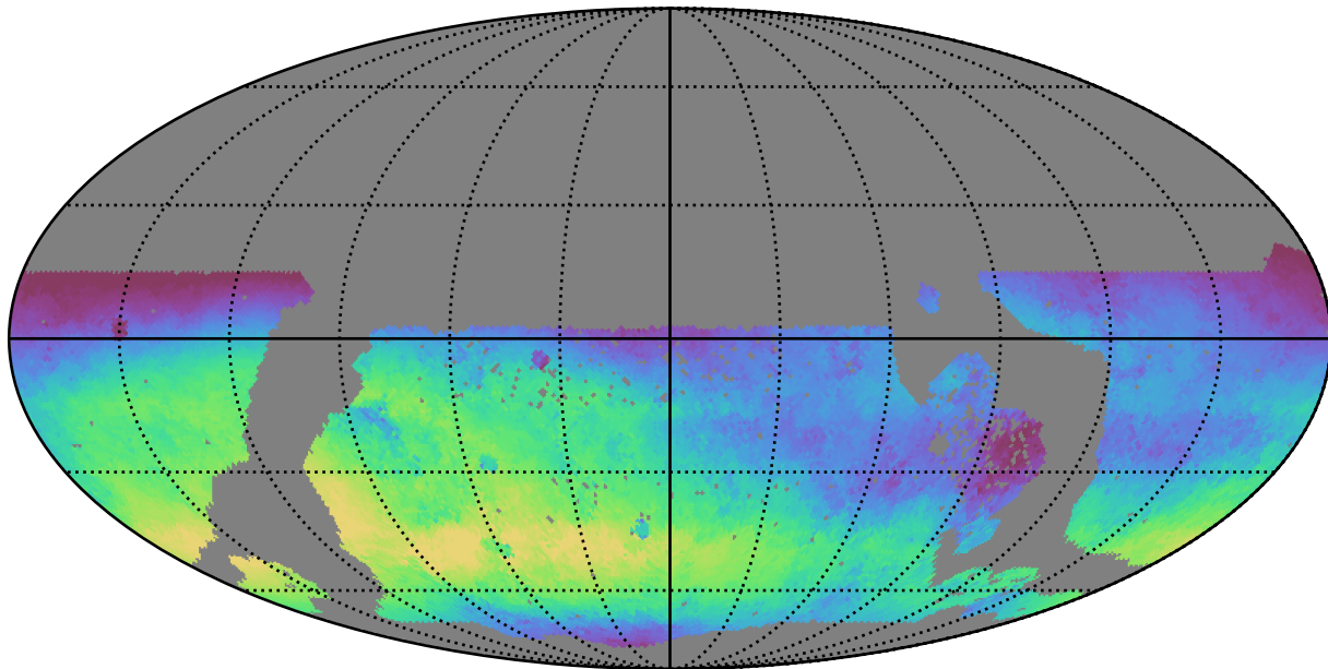
no_magell_roll_v3.4_10yrs WFD u band: Median skyBrightness
