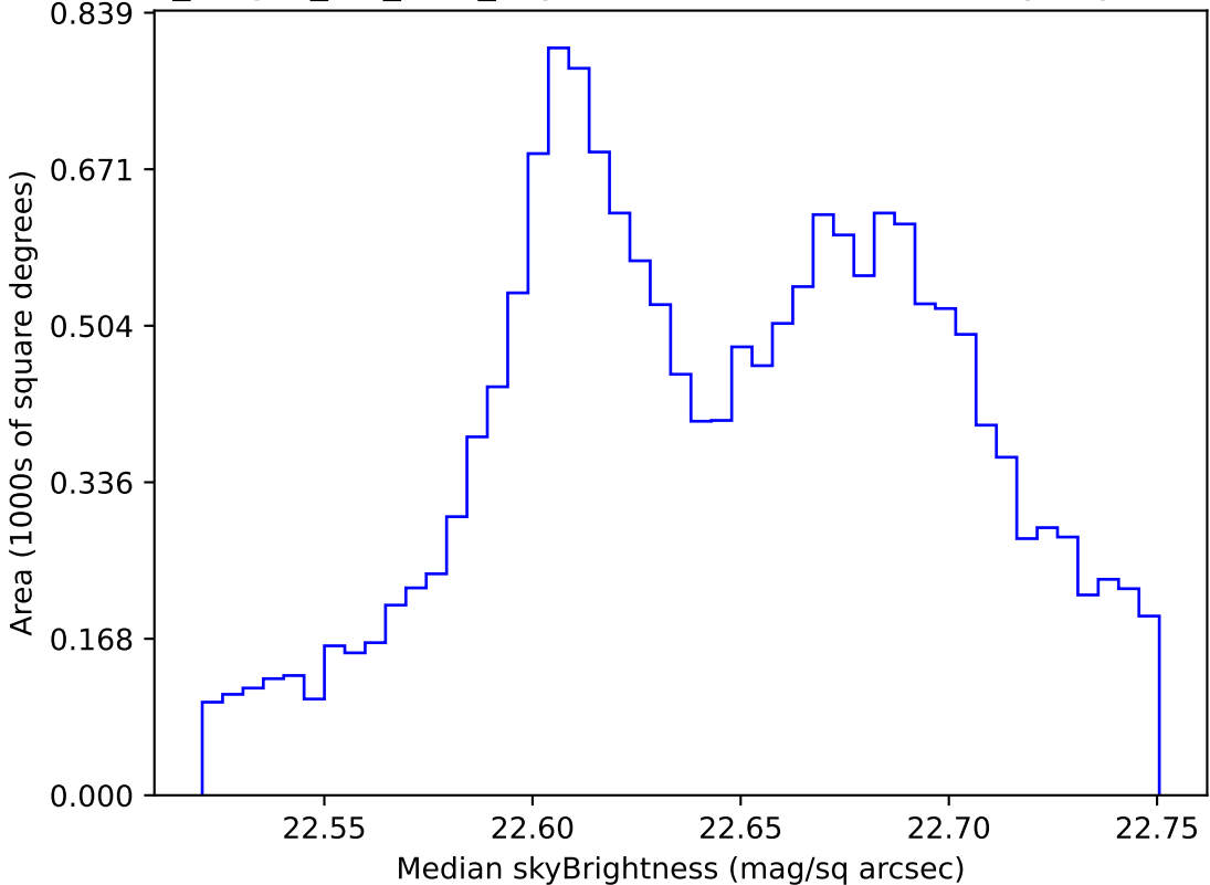
no_magell_roll_v3.4_10yrs WFD u band: Median skyBrightness
