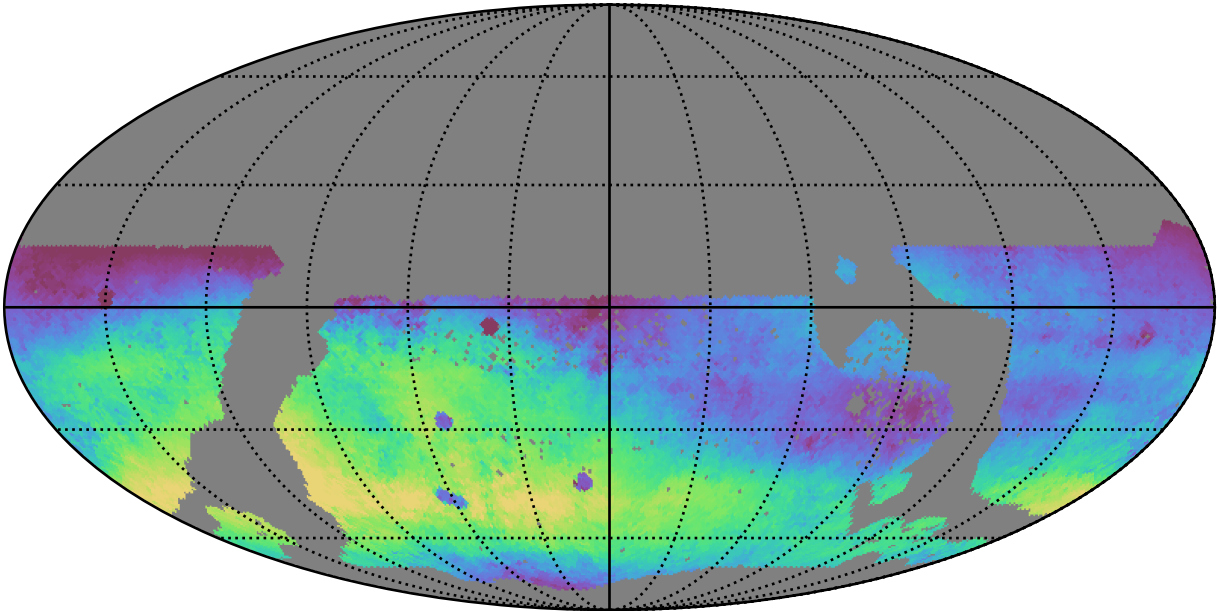
no_magell_roll_v3.4_10yrs WFD r band: Median skyBrightness
