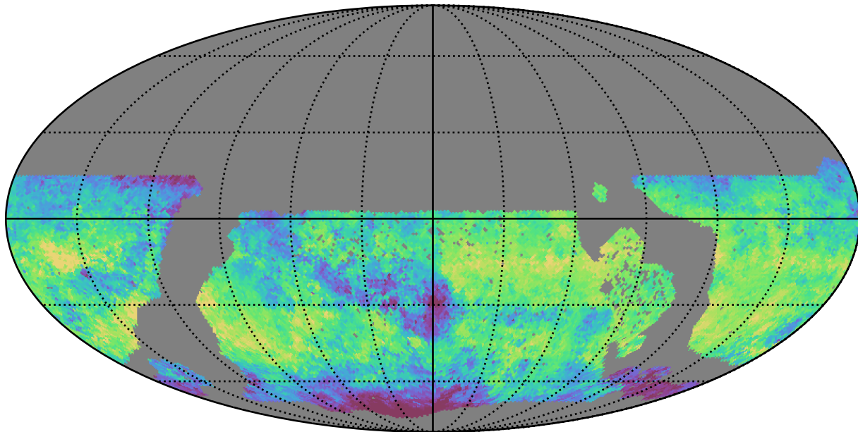
no_magell_roll_v3.4_10yrs WFD i band: Median skyBrightness
