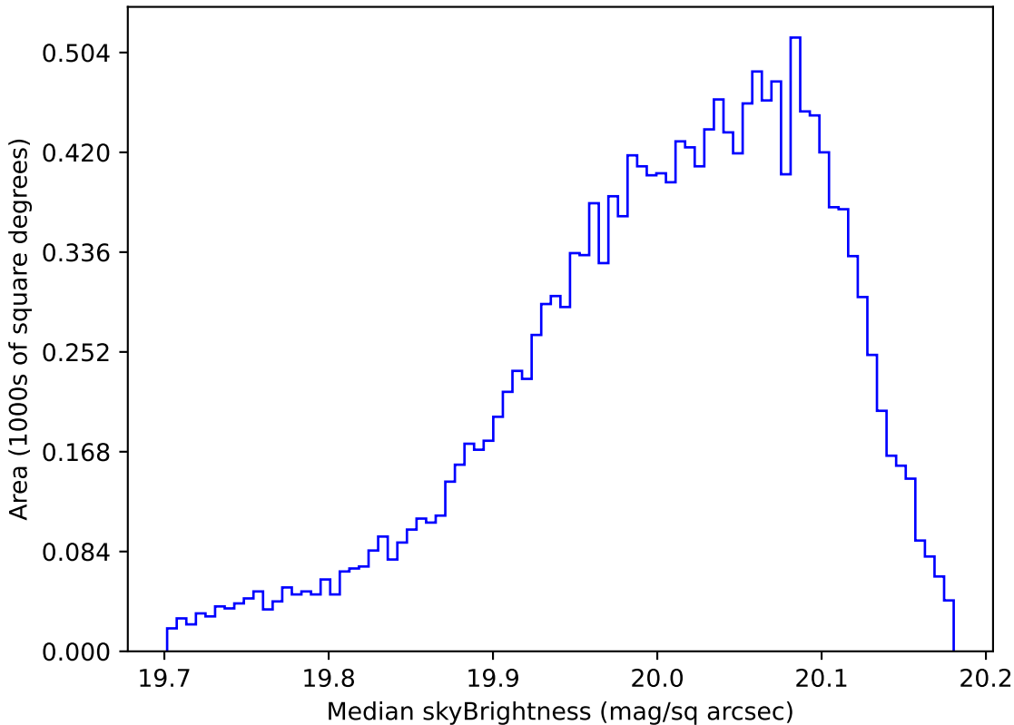
no_magell_roll_v3.4_10yrs WFD i band: Median skyBrightness
