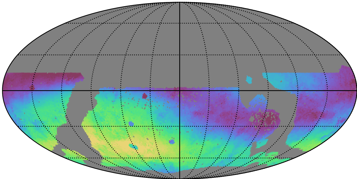
no_magell_roll_v3.4_10yrs WFD g band: Median skyBrightness
