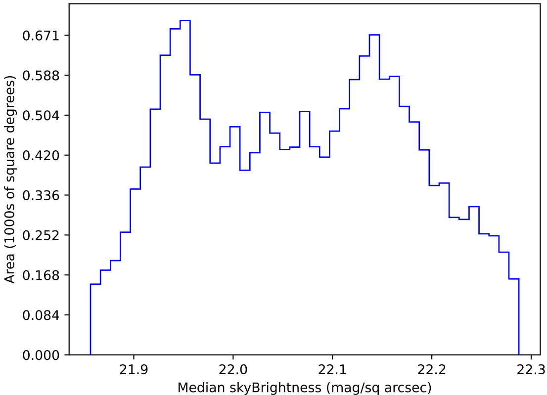
no_magell_roll_v3.4_10yrs WFD g band: Median skyBrightness
