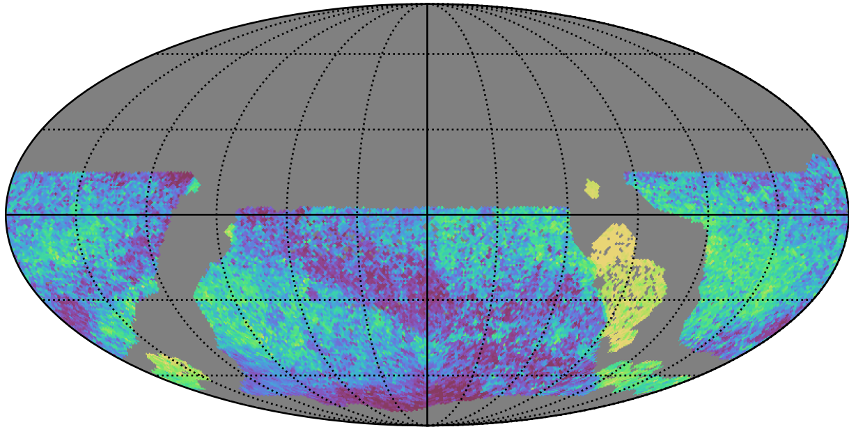
no_magell_roll_v3.4_10yrs WFD all bands: Median skyBrightness
