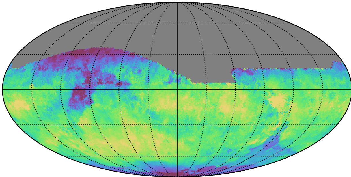
no_magell_roll_v3.4_10yrs All sky z band: Median skyBrightness
