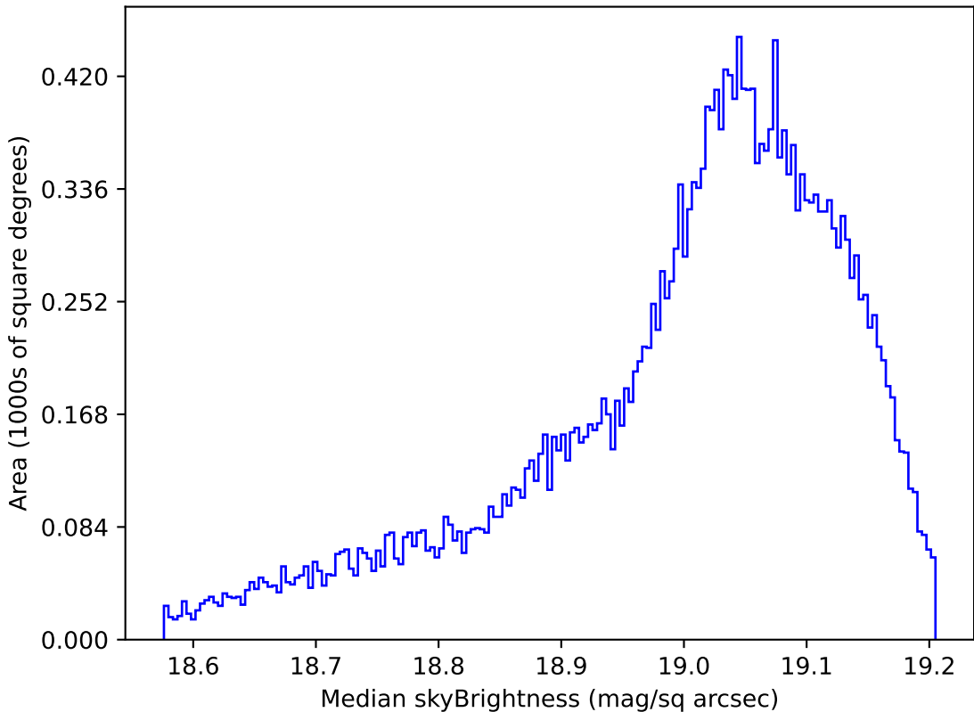
no_magell_roll_v3.4_10yrs All sky z band: Median skyBrightness
