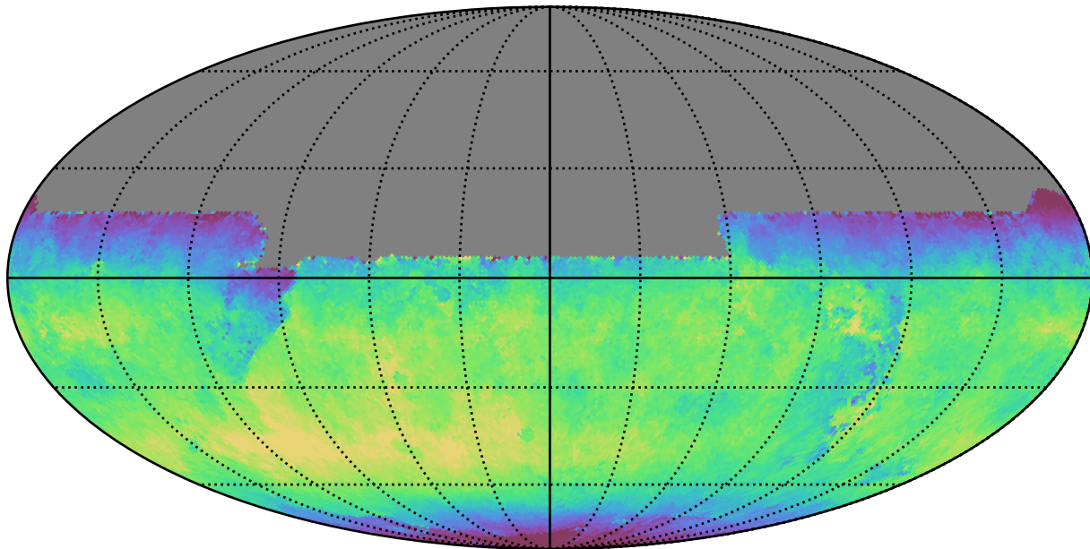
no_magell_roll_v3.4_10yrs All sky y band: Median skyBrightness
